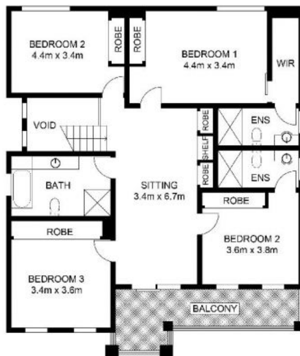
FIRST LEVEL
