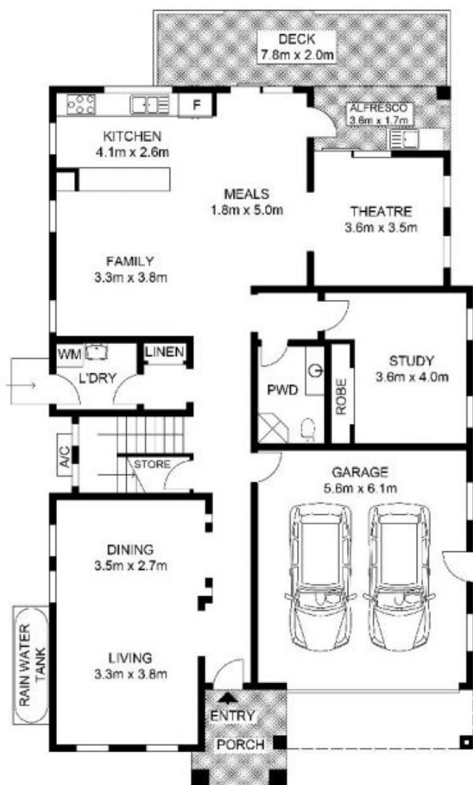
GROUND LEVEL
